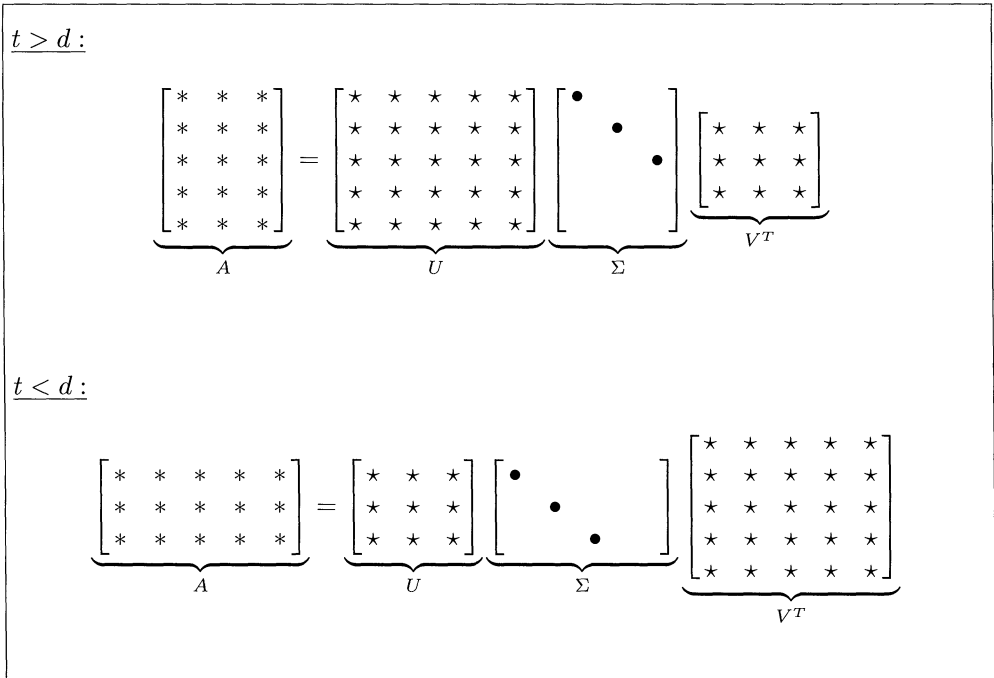
Fig. 5.1 The singular value and singular vector matrices.
