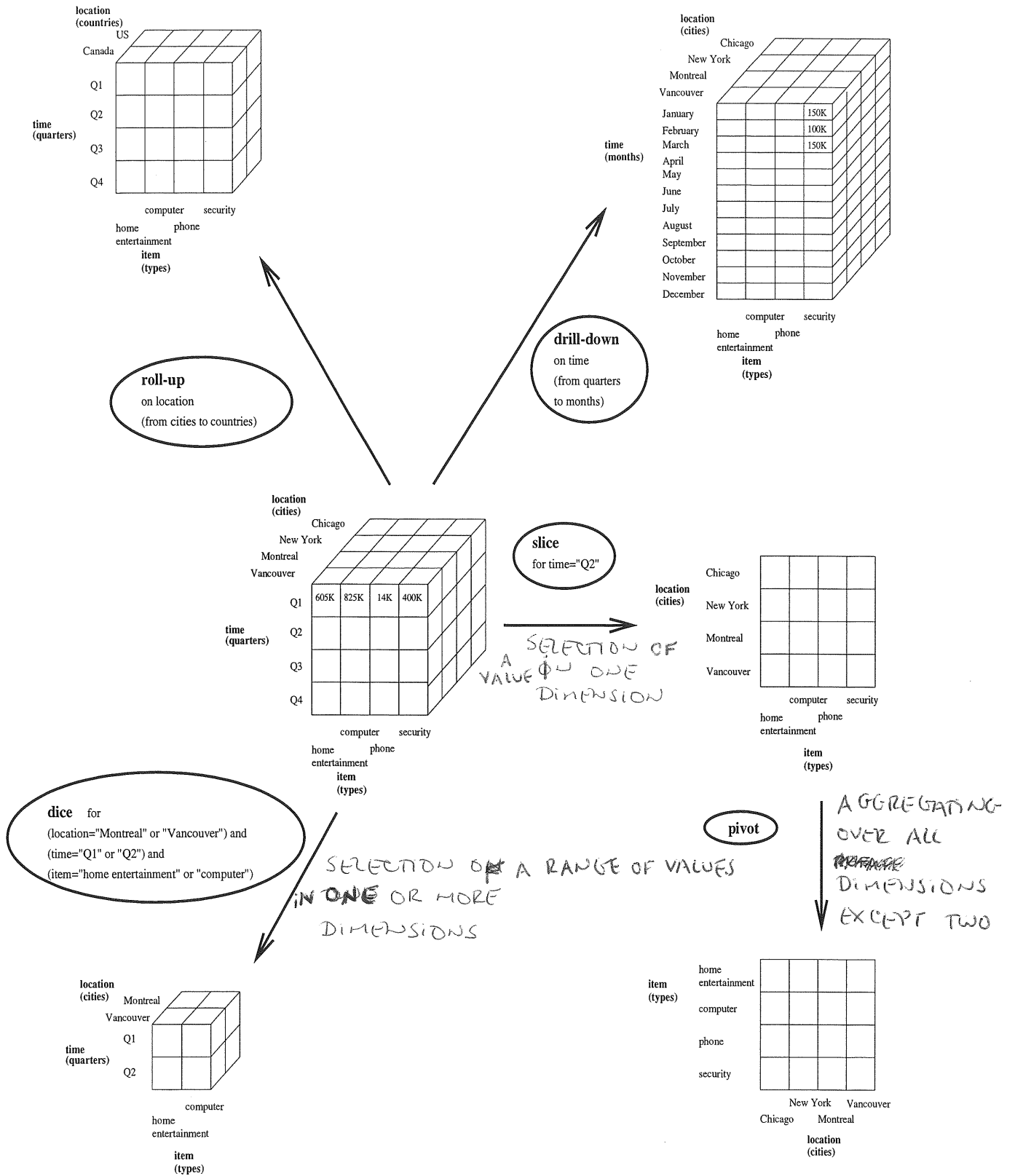
Figure 2.10: Examples of typical OLAP operations on multidimensional data.
