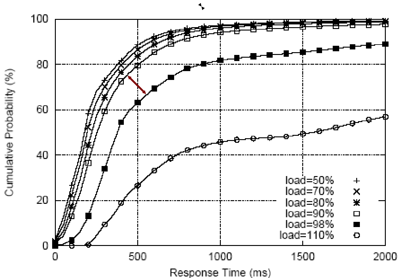
Figure 10: FIFO performance for different loads with a queue length of 120 elements.
