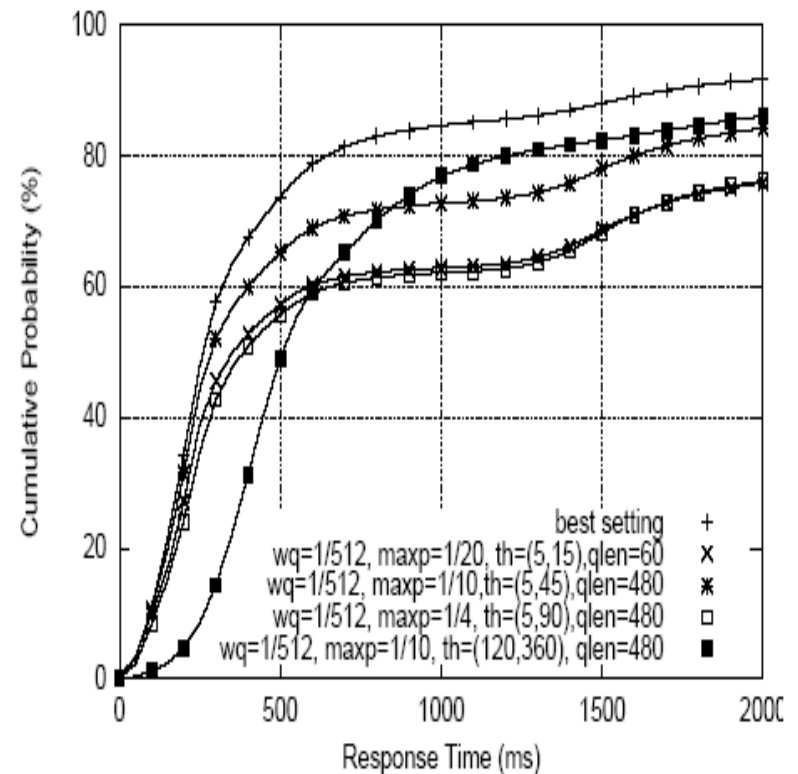
Figure 16b: "Bad" RED parameters settings at 98% load.
