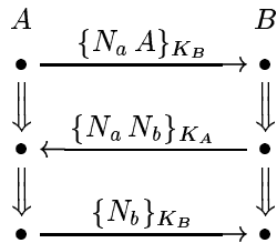
Figure 2: Needham-Schroeder
