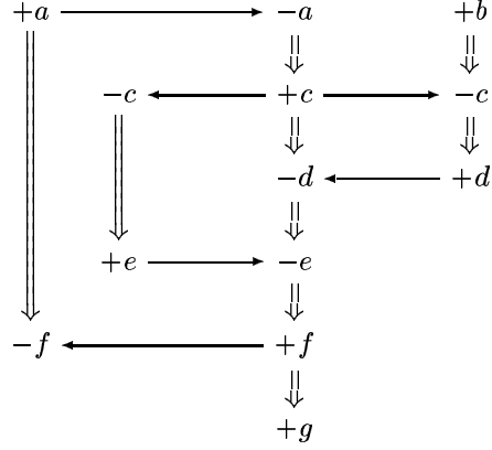
Figure 1: A Bundle
