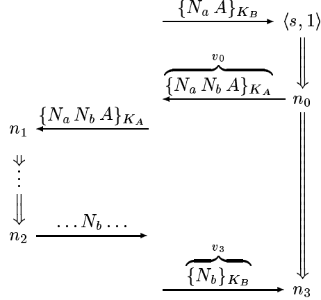
Figure 6: Node n_1 Contains v_0
