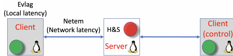
Fig. 3. Hide and Seek computer configuration. Server and clients run Linux and are connected by a high-bitrate LAN. All computers run Hide and Seek, but the server has the authoritative game state. Network latency is added with Linux’s tc with Netem and local latency is added with Evlag.
