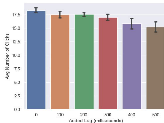
Figure 4.b.2 Sushi Shooter: Click vs Added Lag Bar chart: average click counts with standard error
