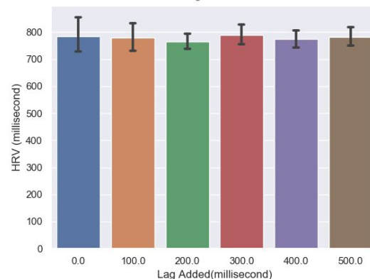
Figure 4.d.4 Square Shooter: HRV vs Added Lag Bar chart: average HRV with standard error
