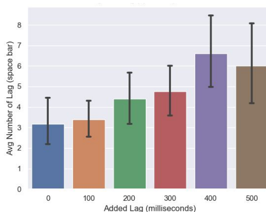
Figure 4.c.6 Square Dodger: Lag (spacebar) vs Added Lag Bar chart: average spacebar counts with standard error
