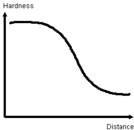
Fig. 7. Jominy end quench graph (Source [3]).
