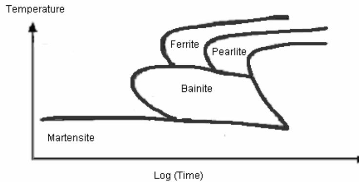
Fig. 6. CCT diagram (Source: Ref. No. [3]).
