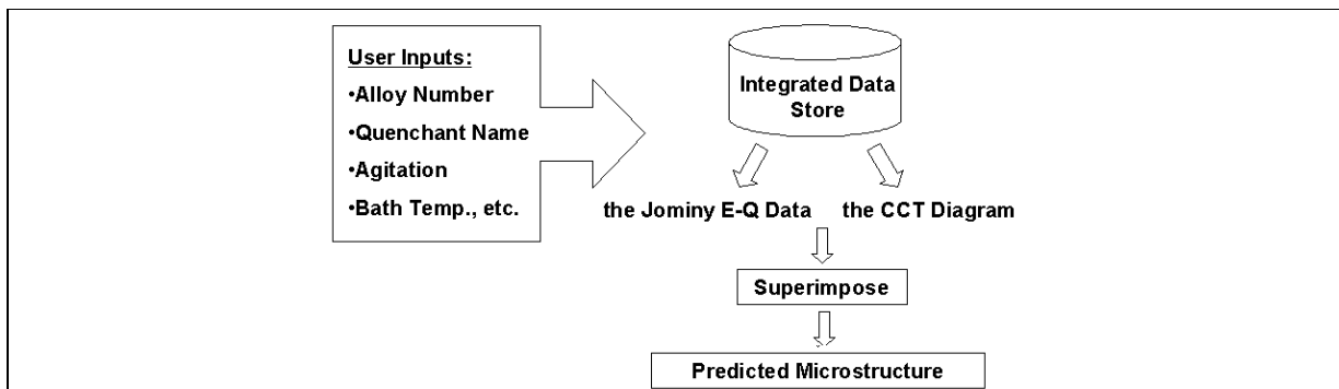
Fig. 8. Microstructure Prediction in QuenchMiner™.
