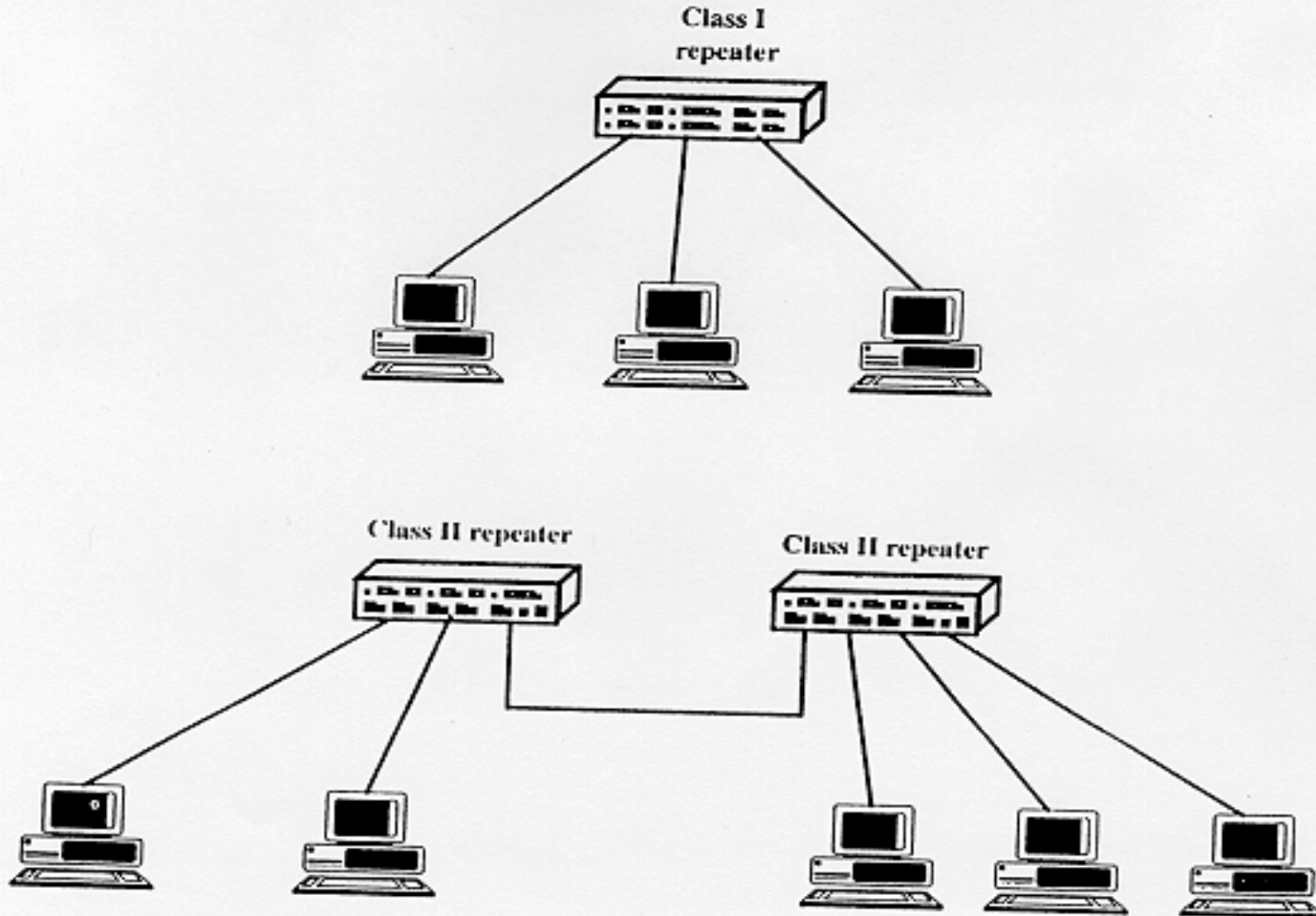
Figure 7.10 100BASE-T Repeater Types
