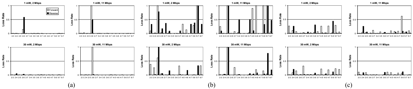
Fig. 5. Loss rate for node pairs for layout1 in (a) ukhome1 , (b) ushome1 , (c) ushome2 .
