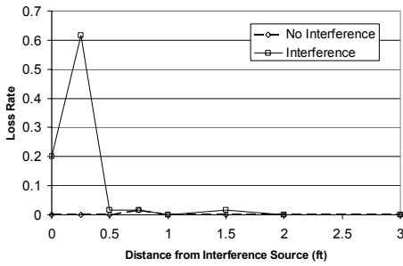
Fig. 10. The impact of a 600W microwave on a receiver at varying distance from the interference source and a distance of 15 feet from the sending node.
