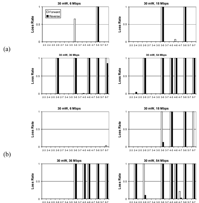
Fig. 12. Loss rate for each pair of nodes for ushome2 using IEEE 802.11a, for two different node orientations, (a) layout1 and (b) layout2 .
