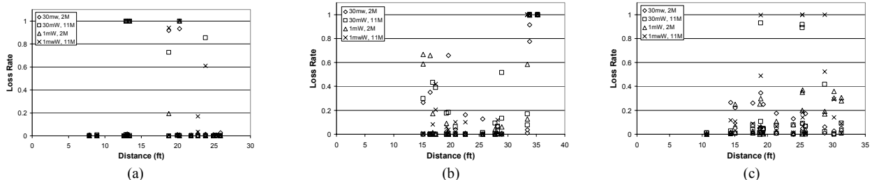
Fig. 9. Loss rate for each pair of nodes against their distance for (a) ukhome1 , (b) ushome1 and (c) ushome2 under layout2
