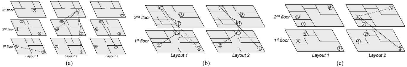
Fig. 7. Abstract home floorplans and location of links with greater than 95% loss rate at 1 mW and 11 Mbps under different configurations: (a) ukhome1 for layout1 , layout2 , and layout3 , (b) ushome1 , and (c) ushome2 for layout1 and layout2 . Dashed lines indicate asymmetric links.
