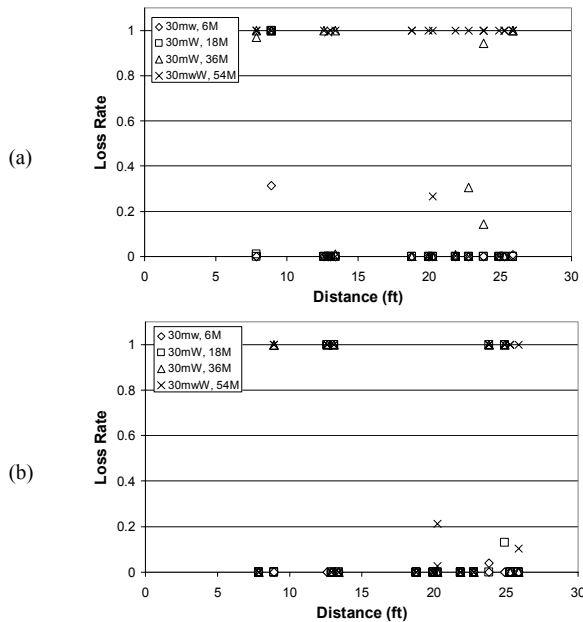
Fig. 13. Loss rate for each pair of nodes versus their physical distance under IEEE 802.11a ( layout2 ) for (a) ushome1 and (b) ushome2 .
