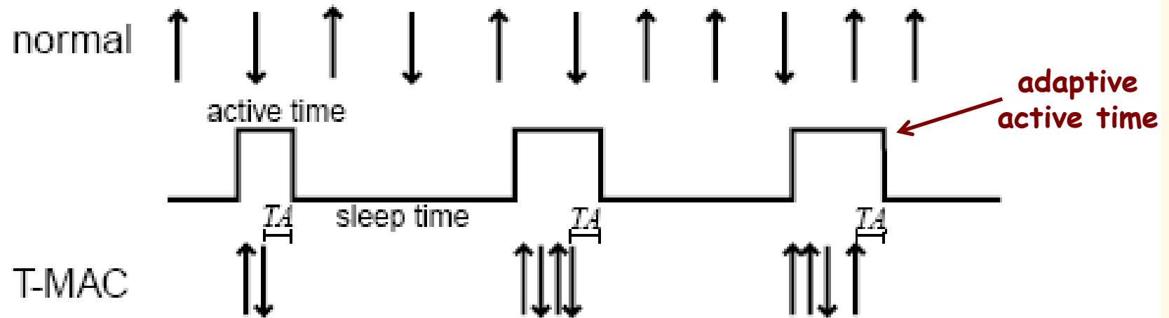
Figure 2: The basic T-MAC protocol scheme, with adaptive active times.
