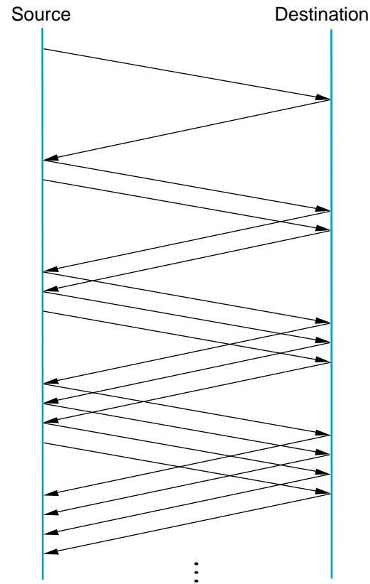
Figure 6.8 Additive Increase
