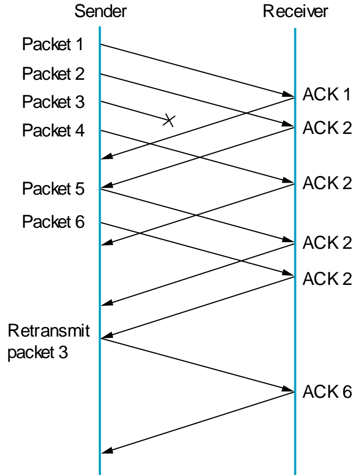
Figure 6.12 Fast Retransmit
