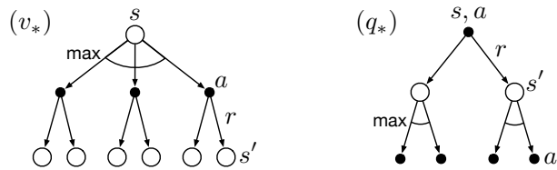
Figure 3.5: Backup diagrams for v_* and q_*
