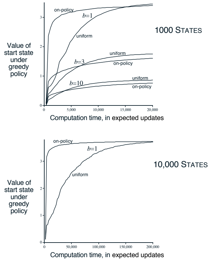
Figure 8.9: Relative efficiency of updates distributed uniformly across the state space versus focused on simulated on-policy trajectories, each starting in the same state. Results are for randomly generated tasks of two sizes and various branching factors, b .
