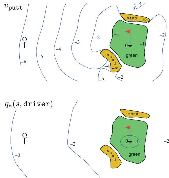
Figure 3.4: A golf example: the state-value function for putting (upper) and the optimal action-value function for using the driver (lower). ■
