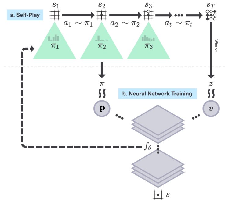
Figure 16.8: AlphaGo Zero self-play reinforcement learning. a) The program played many games against itself, one shown here as a sequence of board positions s_i , i = 1, 2, \dots, T , with moves a_i , i = 1, 2, \dots, T , and winner z . Each move a_i was determined by action probabilities \pi_i returned by MCTS executed from root node s_i and guided by a deep convolutional network, here labeled f_\theta , with latest weights \theta . Shown here for just one position s but repeated for all s_i , the network’s inputs were raw representations of board positions s_i (together with several past position, though not shown here), and its outputs were vectors \mathbf{p} of move probabilities that guided MCTS’s forward searches, and scalar values v that estimated the probability of the current player winning from each position s_i . b) Deep convolutional network training. Training examples were randomly sampled steps from recent self-play games. Weights \theta were updated to move the policy vector \mathbf{p} toward the probabilities \pi returned by MCTS, and to include the winners z in the estimated win probability v . Reprinted from draft of Silver et al. (2017) with permission of the authors and DeepMind.
