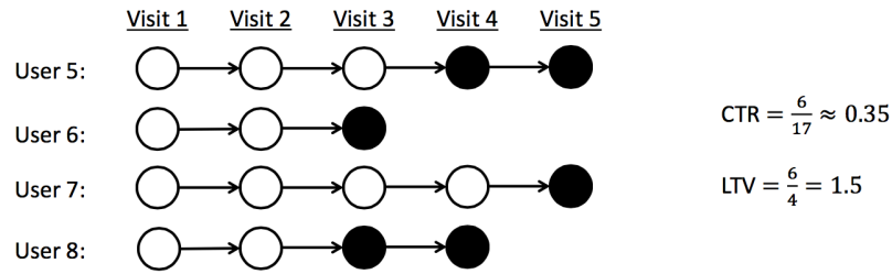
Figure 16.9: Click through rate (CTR) versus life-time value (LTV). Each circle represents a user visit; black circles are visits at which the user clicks. Adapted from Theocharous et al. (2015).
