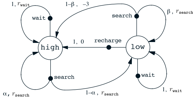
Figure 3.2: Transition graph for the recycling robot example.
