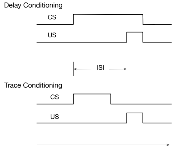
Figure 14.1: Arrangement of stimuli in two types of classical conditioning experiments. In delay conditioning, the CS extends throughout the interstimulus interval, or ISI, which is the time interval between the CS onset and the US onset (often with the CS and US ending at the same time as shown here). In trace conditioning, there is a time interval, called the trace interval, between CS offset and US onset.
