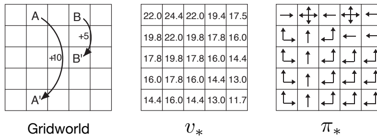
Figure 3.6: Optimal solutions to the gridworld example.
