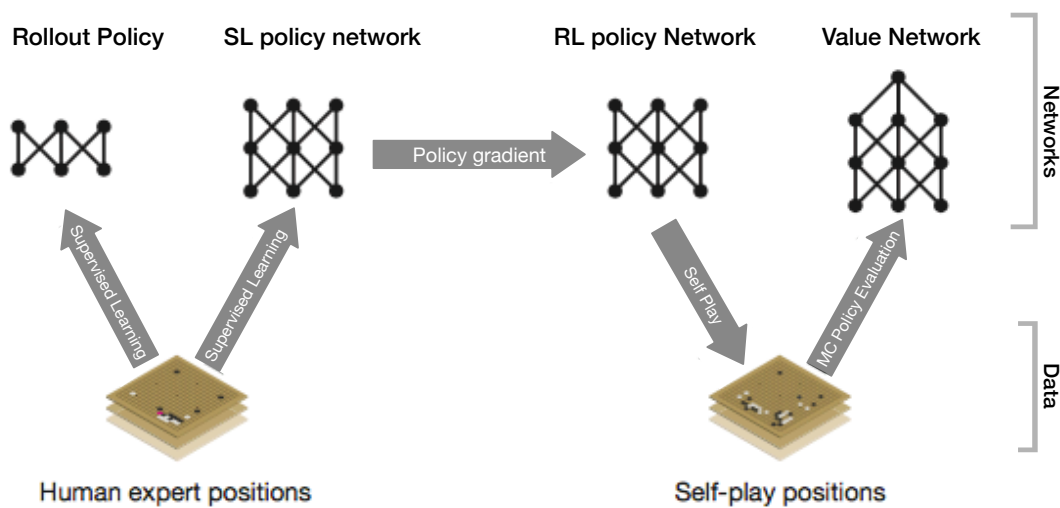
Figure 16.7: AlphaGo pipeline. Adapted with permission from Macmillan Publishers Ltd: Nature , vol. 529(7587), p. 485, copyright (2016).
