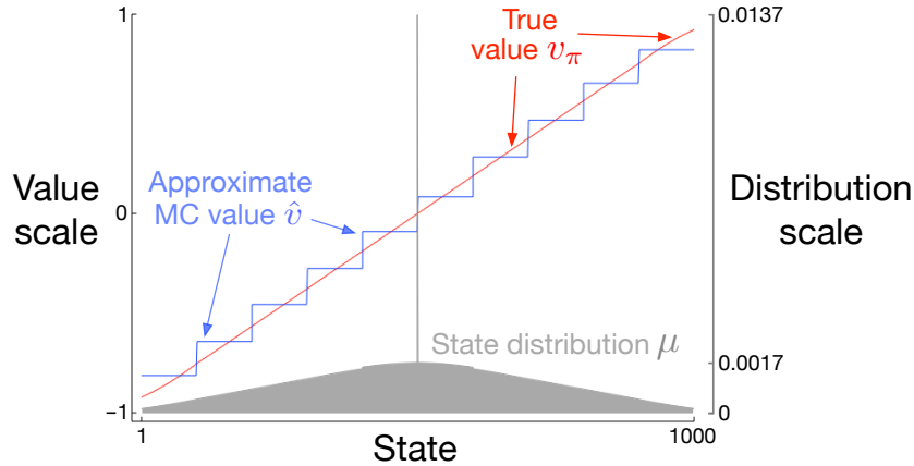
Figure 9.1: Function approximation by state aggregation on the 1000-state random walk task, using the gradient Monte Carlo algorithm (page 165). ■
