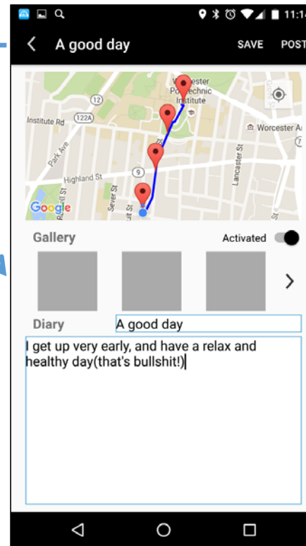
DiaryDetailActivity
