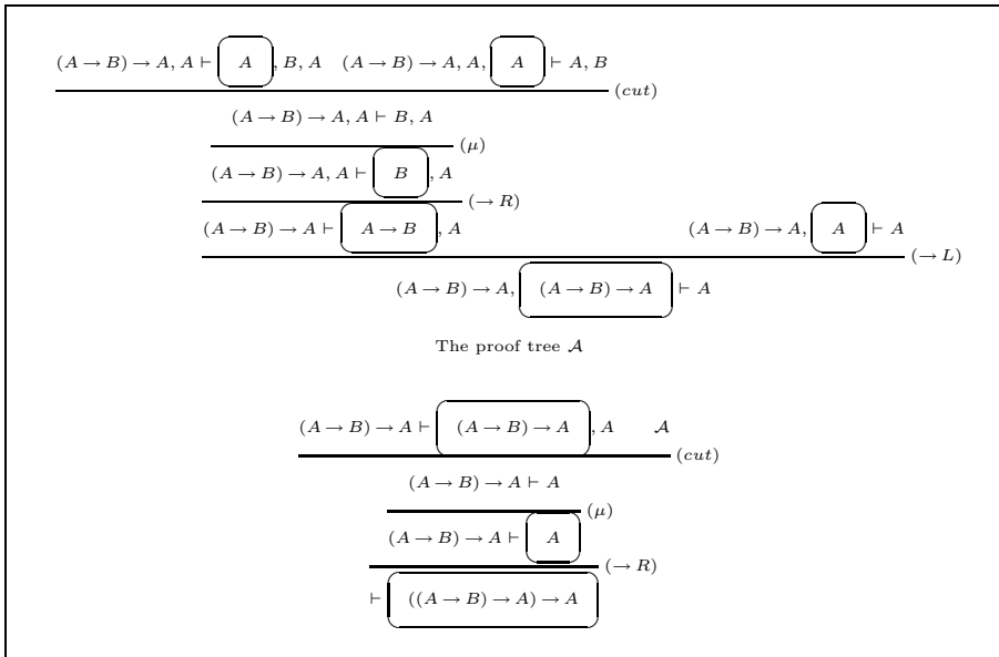
Fig. 2. Peirce’s law with active formula
