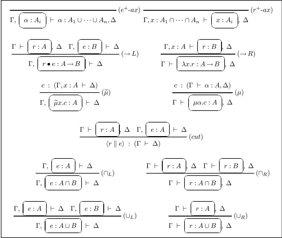
Fig. 5. The system \mathcal{M}^{\cap \cup}
