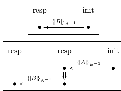
Figure 9: Reflect Protocol and Shapes
