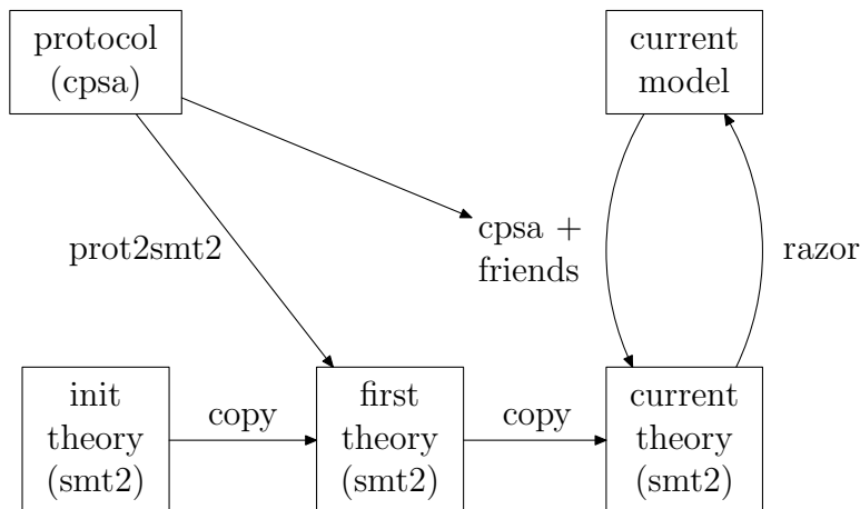
Figure 1: LPA Architecture
