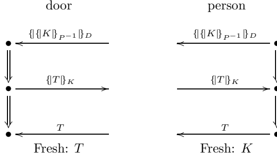
Figure 5: DoorSEP Protocol
