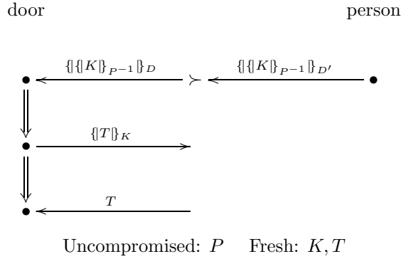
Figure 7: DoorSEP First Shape
