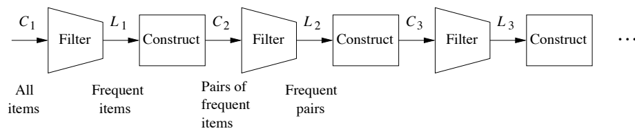
Figure 6.4: The A-Priori Algorithm alternates between constructing candidate sets and filtering to find those that are truly frequent
