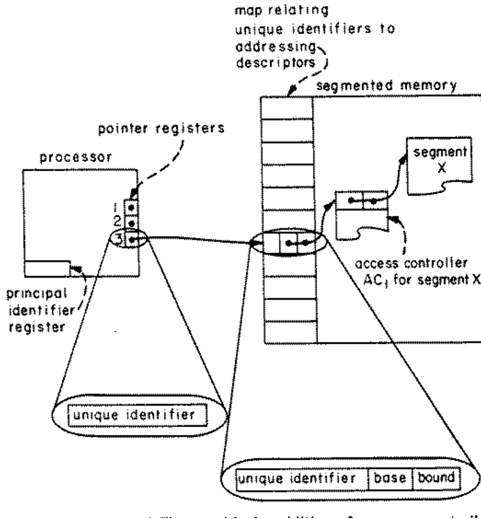
Fig. 9. A revision of Fig. 5, with the addition of an access controller as an indirect address to be used on all references by the processor to the memory. Since the access controller contains permission bits, they no longer need appear in the processor registers, which have been renamed "pointer" registers. Note that the privileged state bit of the processor has been replaced with a principal identifier register.
