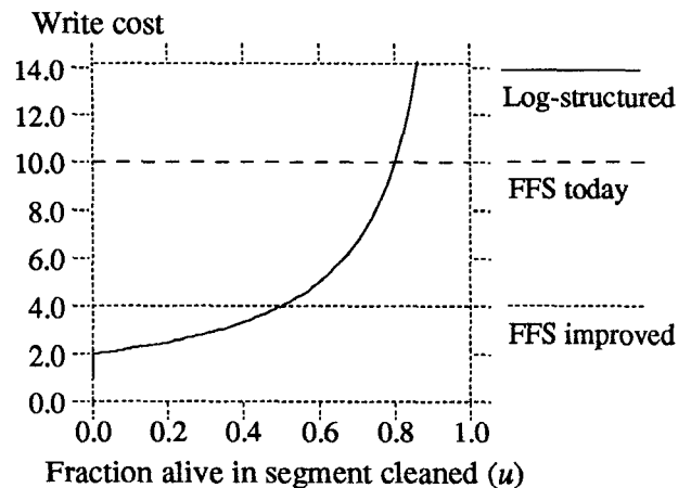
Figure 3 — Write cost as a function of u for small files. In a log-structured file system, the write cost depends strongly on the utilization of the segments that are cleaned. The more live data in segments cleaned the more disk bandwidth that is needed for cleaning and not available for writing new data. The figure also shows two reference points: "FFS today", which represents Unix FFS today, and "FFS improved", which is our estimate of the best performance possible in an improved Unix FFS. Write cost for Unix FFS is not sensitive to the amount of disk space in use.
