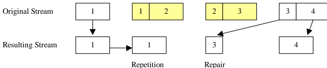
Figure 1.1 Our Approach – Combine Media Specific Forward Error Correction and Packet Repetition
