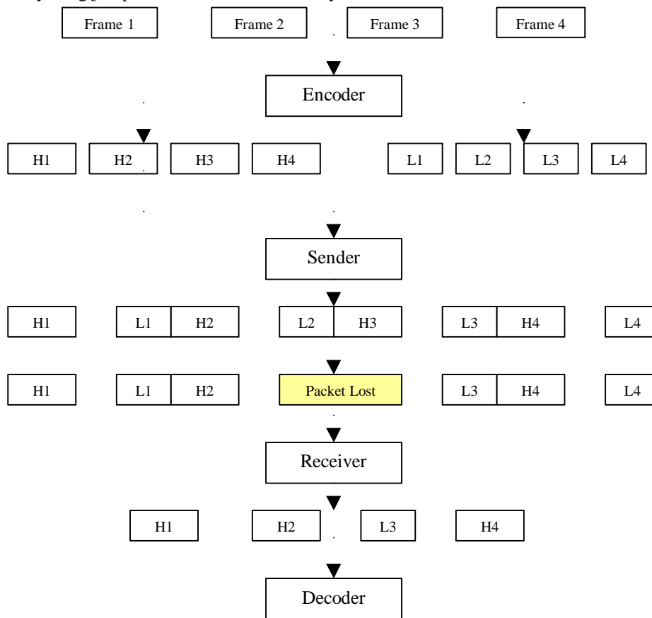
Figure 3.1. Video Redundancy Architecture
