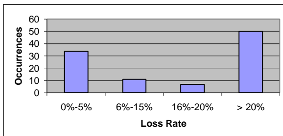
Figure 3.2.a Loss Rate Distribution
