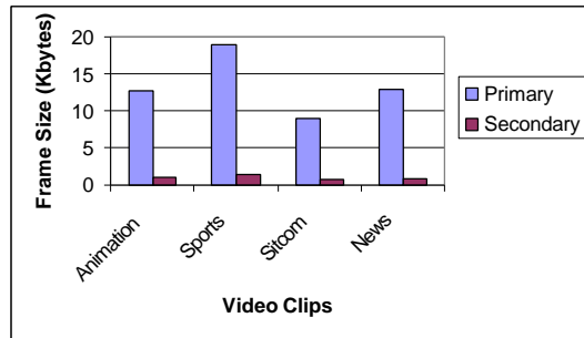
Figure 4.1.2 Frame Size Differences for Four Videos
