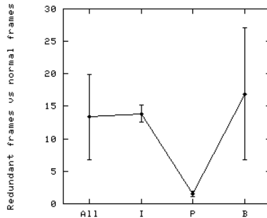
Figure 4.1.3 Ratios of Overhead versus Frame Size
