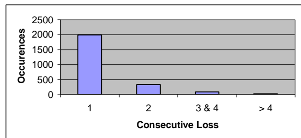
Figure 3.2.b Consecutive Loss Distribution
