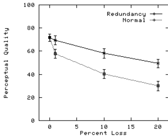
Figure 3.4 Effects of Loss Rate to Perceptual Quality
