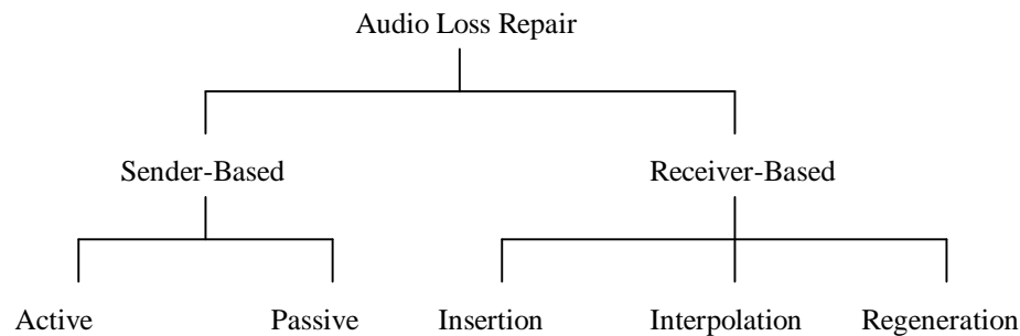
Figure 2.1 Taxonomy of Audio Loss Repair Techniques
