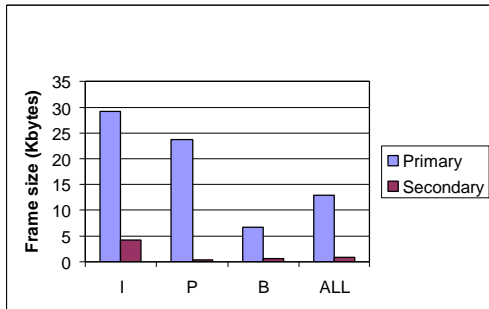
Figure 4.1.1 Frame Size Differences for Primary Frames and Secondary Frames
