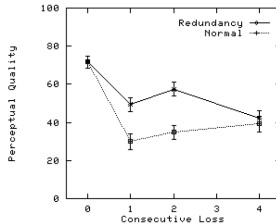
Figure 3.5 Effects of Loss Pattern to Perceptual Quality
