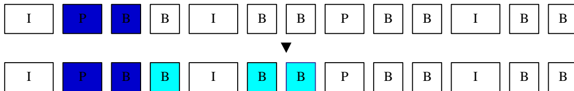
Figure 3.6.a Two Consecutive Frame Losses
