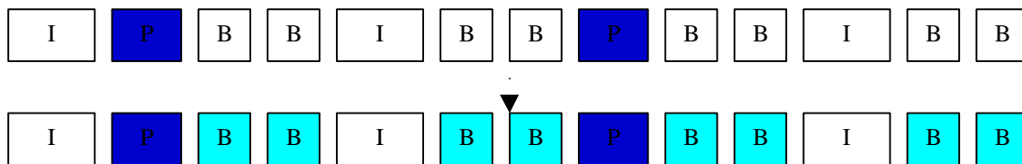
Figure 3.6.b Two Single Frame Losses
